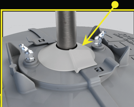
SELF-CENTERING LID
